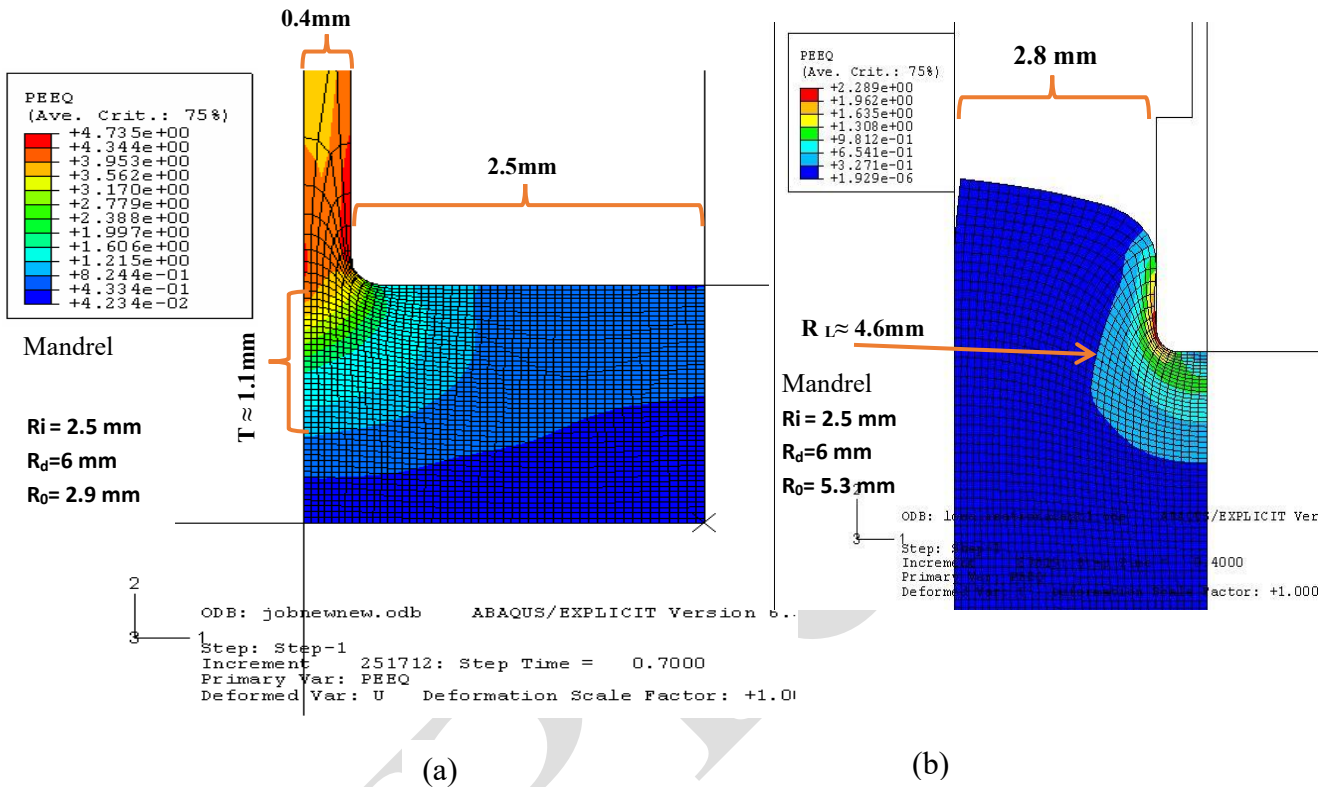
Figure 11: Equivalent plastic strain distribution from FEM simulations for (a) 400 \mu m wall thickness (uniform deformation, no localization) and (b) 2.8 mm wall thickness (localized shear near outer radius).
